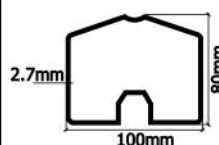
Eave Purlin
