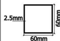
Roof Purlin
